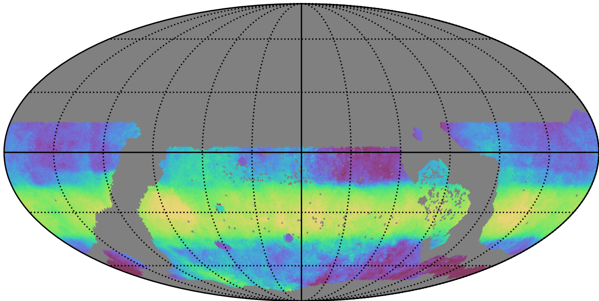
ddf_acor_sf15_lsf20_lsr50_v3.4_10yrs WFD i band: Median HA
