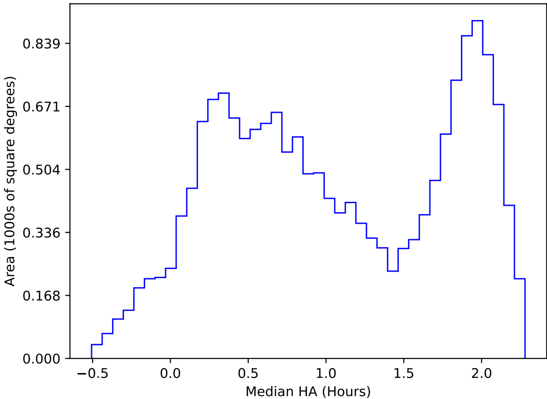
ddf_acor_sf15_lsf20_lsr50_v3.4_10yrs WFD i band: Median HA
