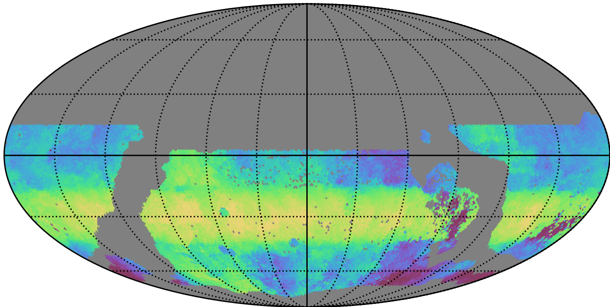
ddf_acor_sf15_lsf20_lsr50_v3.4_10yrs WFD g band: Median HA
