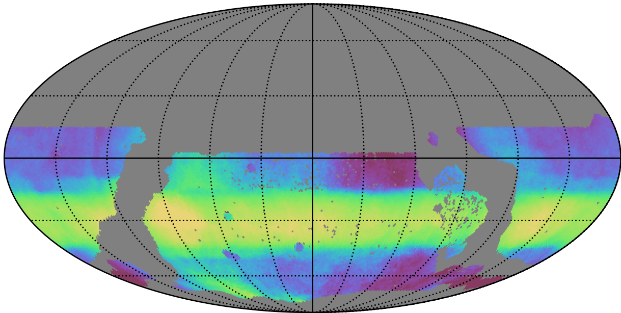
ddf_acor_sf15_lsf20_lsr50_v3.4_10yrs WFD all bands: Median HA
