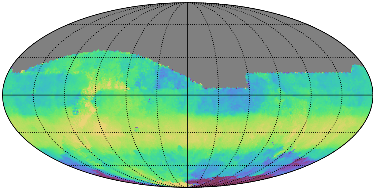
ddf_acor_sf15_lsf20_lsr50_v3.4_10yrs All sky z band: Median HA
