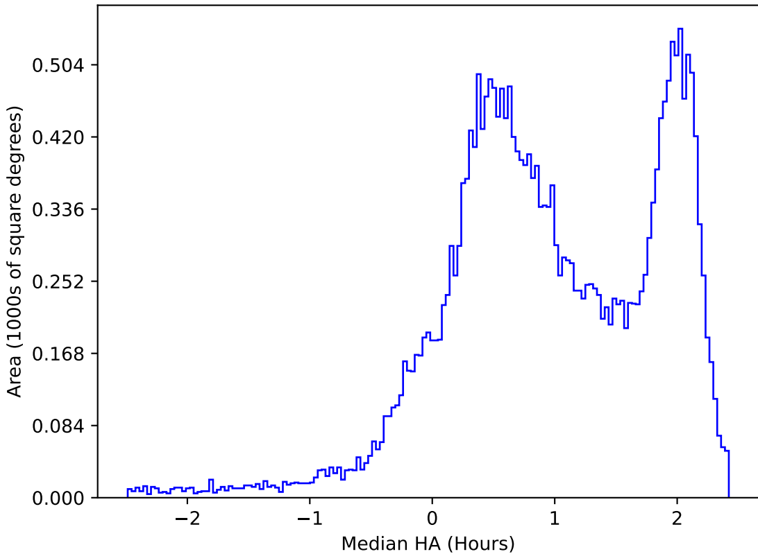
ddf_acor_sf15_ls20_lsr50_v3.4_10yrs All sky z band: Median HA
