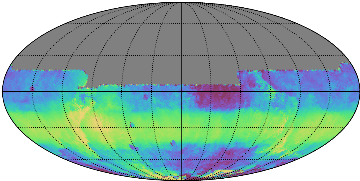
ddf_acor_sf15_lsf20_lsr50_v3.4_10yrs All sky y band: Median HA
