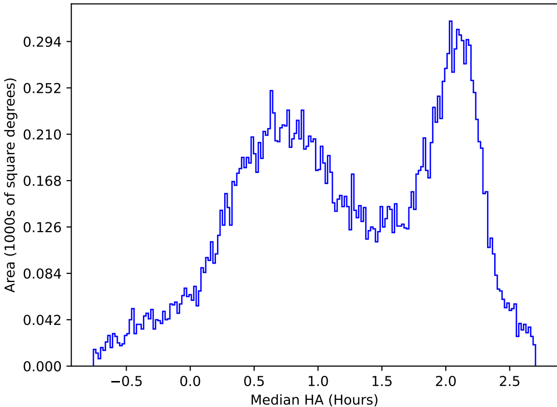
ddf_acor_sf15_ls20_lsr50_v3.4_10yrs All sky y band: Median HA
