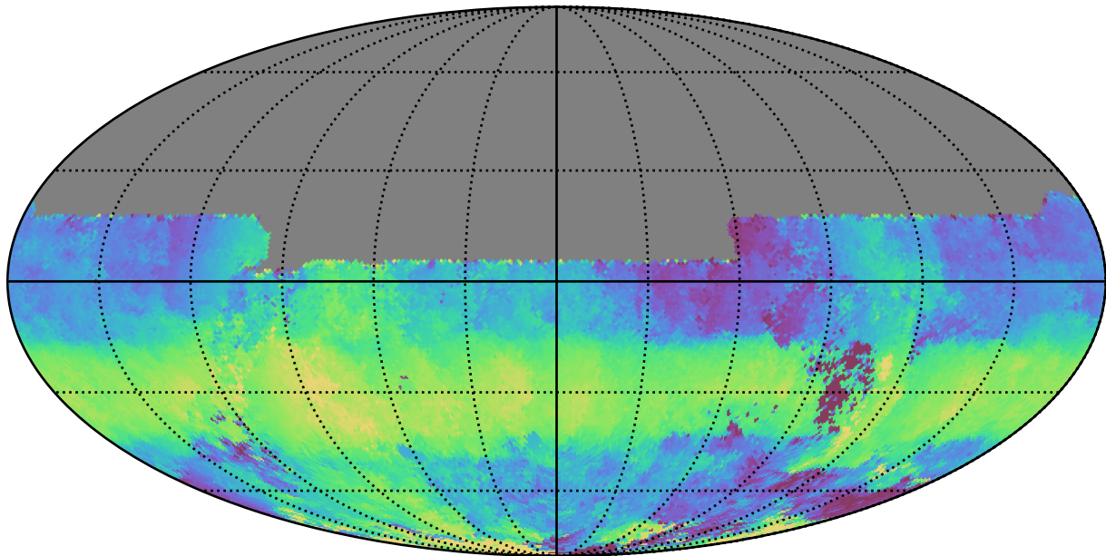
ddf_acor_sf15_lsf20_lsr50_v3.4_10yrs All sky u band: Median HA
