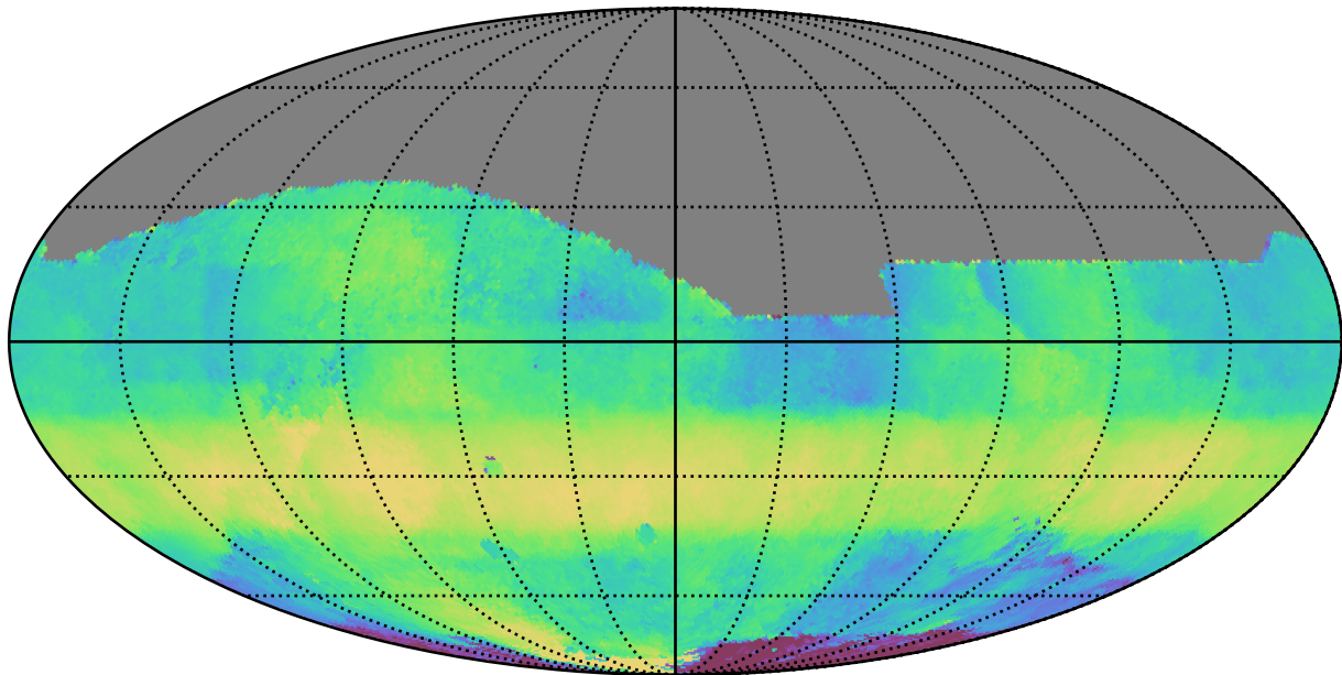
ddf_acor_sf15_lsf20_lsr50_v3.4_10yrs All sky r band: Median HA
