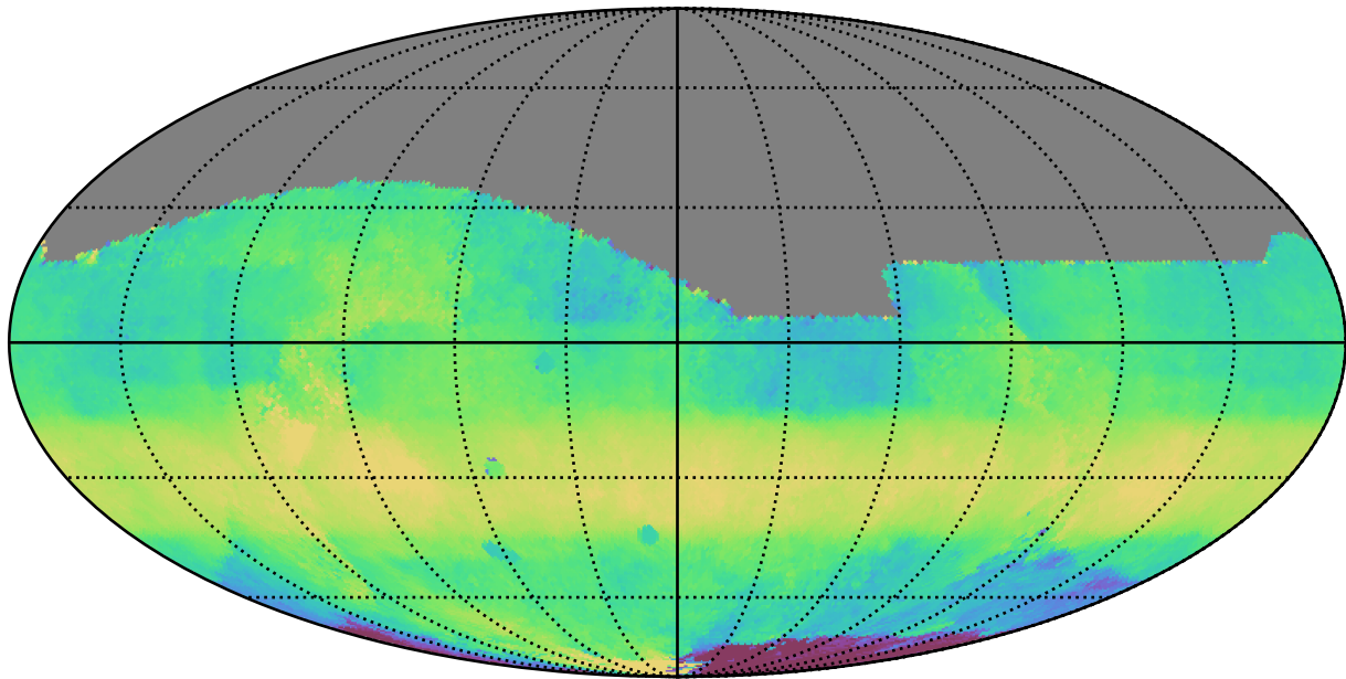
ddf_acor_sf15_lsf20_lsr50_v3.4_10yrs All sky i band: Median HA
