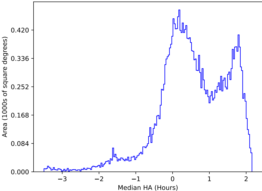
ddf_acor_sf15_lsf20_lsr50_v3.4_10yrs All sky g band: Median HA
