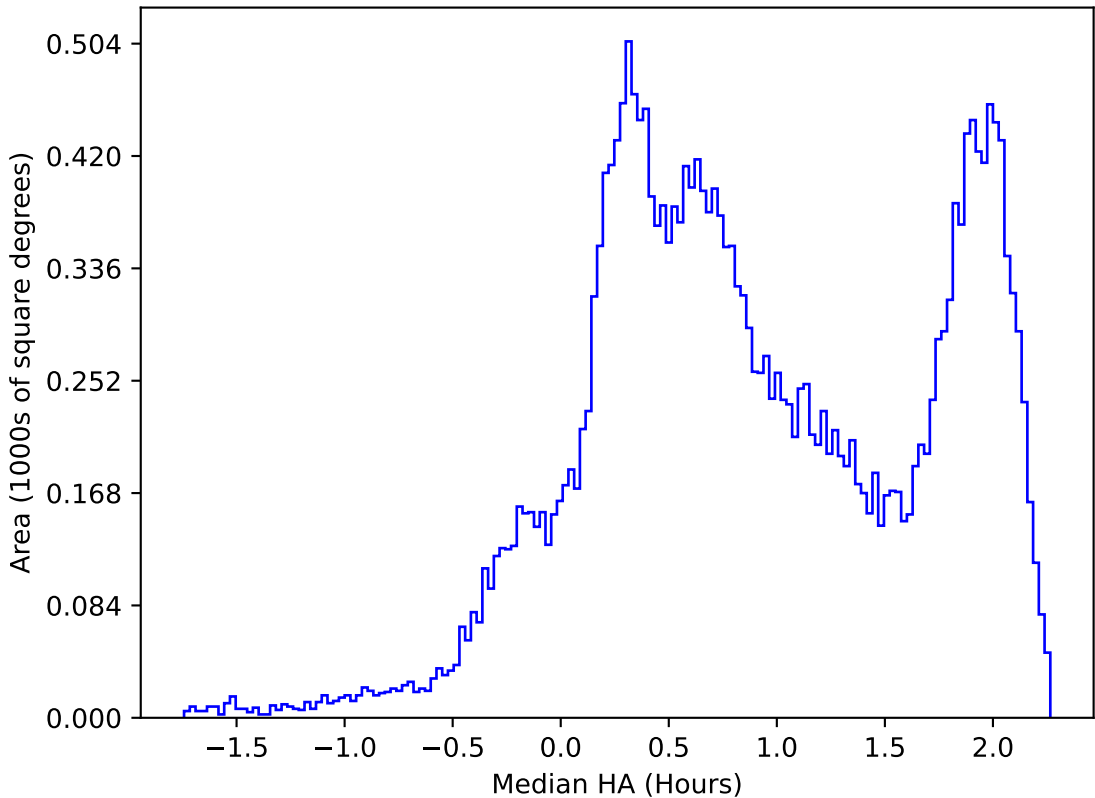
ddf_acor_sf15_lsf20_lsr50_v3.4_10yrs All sky all bands: Median HA
