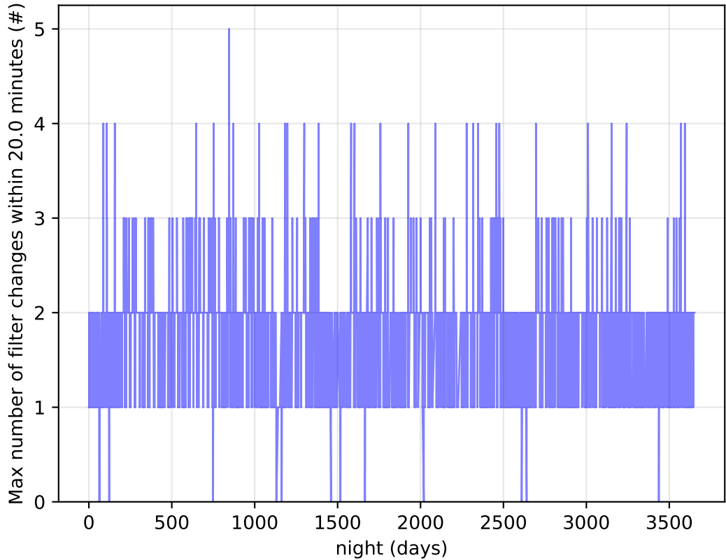
ddf_acor_sf15_Isf20_Isr50_v3.4_10yrs Per Night: Max number of filter changes within 20.0 minutes
