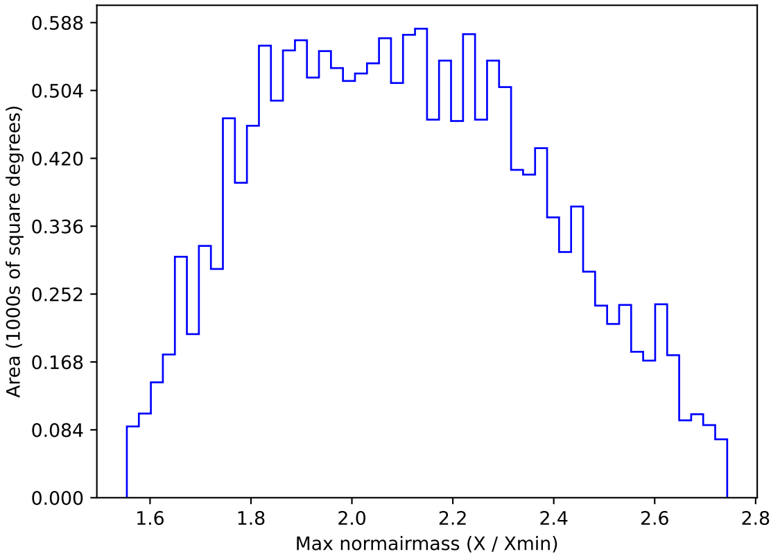
ddf_acor_sf15_lsf20_lsr50_v3.4_10yrs WFD y band: Max normairmass
