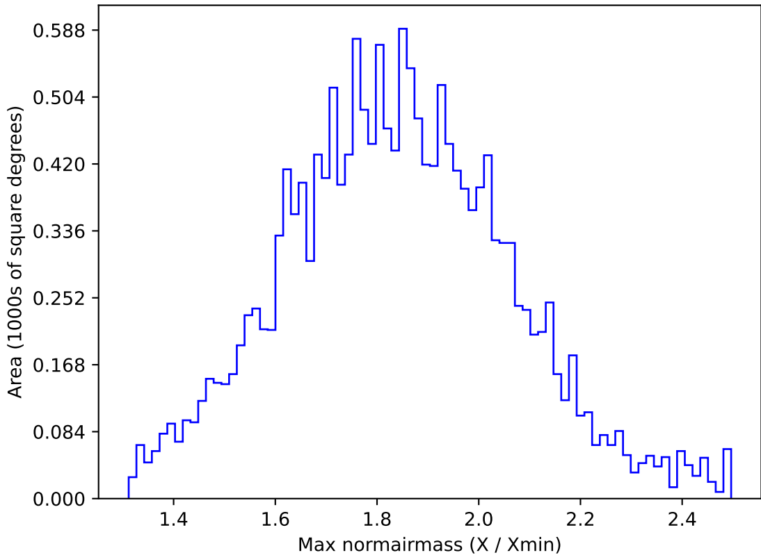
ddf_acor_sf15_lsf20_lsr50_v3.4_10yrs WFD g band: Max normairmass
