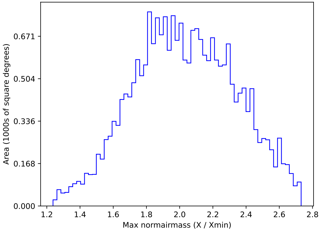
ddf_acor_sf15_lsf20_lsr50_v3.4_10yrs All sky y band: Max normairmass
