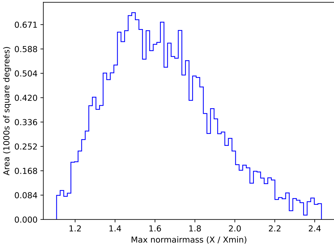
ddf_acor_sf15_lsf20_lsr50_v3.4_10yrs All sky u band: Max normairmass
