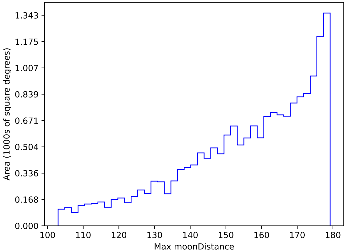
ddf_acor_sf15_lsf20_lsr50_v3.4_10yrs WFD i band: Max moonDistance
