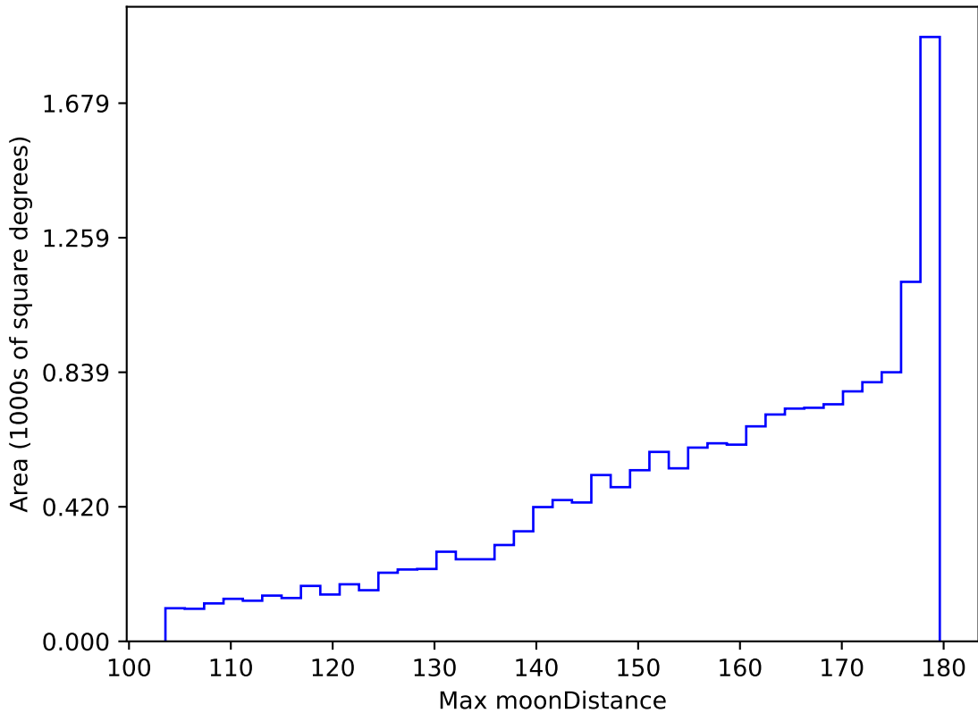
ddf_acor_sf15_lsf20_lsr50_v3.4_10yrs WFD all bands: Max moonDistance
