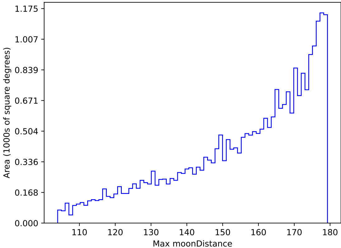
ddf_acor_sf15_lsf20_lsr50_v3.4_10yrs All sky r band: Max moonDistance
