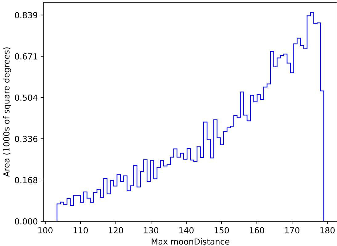
ddf_acor_sf15_lsf20_lsr50_v3.4_10yrs All sky g band: Max moonDistance
