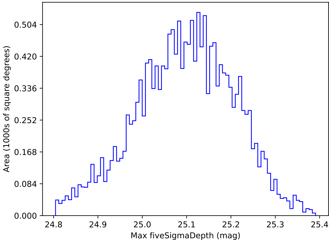
ddf_acor_sf15_lsf20_lsr50_v3.4_10yrs WFD all bands: Max fiveSigmaDepth
