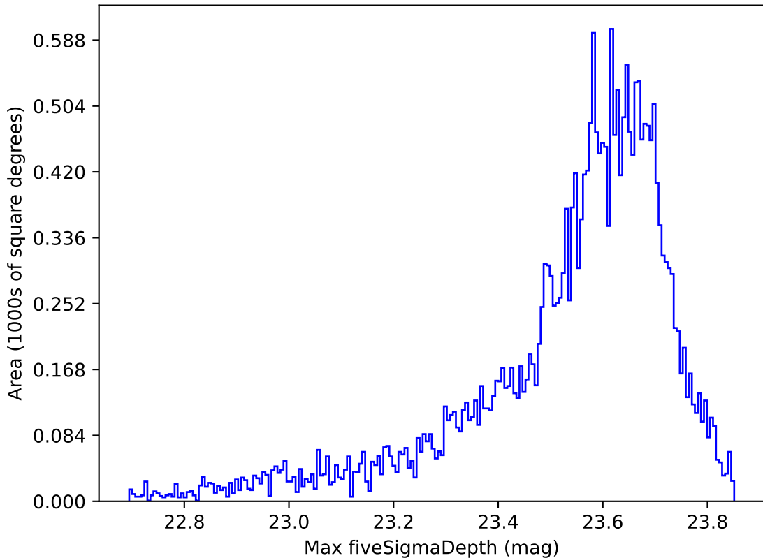
ddf_acor_sf15_lsf20_lsr50_v3.4_10yrs All sky z band: Max fiveSigmaDepth
