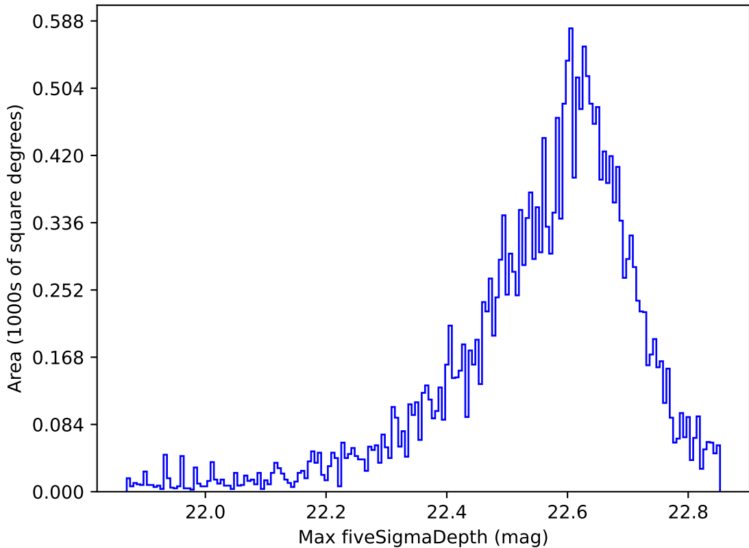
ddf_acor_sf15_ls20_lsr50_v3.4_10yrs All sky y band: Max fiveSigmaDepth
