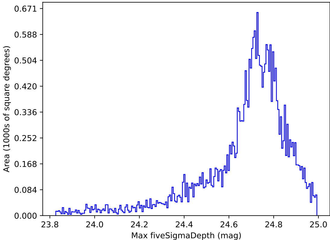
ddf_acor_sf15_lsf20_lsr50_v3.4_10yrs All sky r band: Max fiveSigmaDepth
