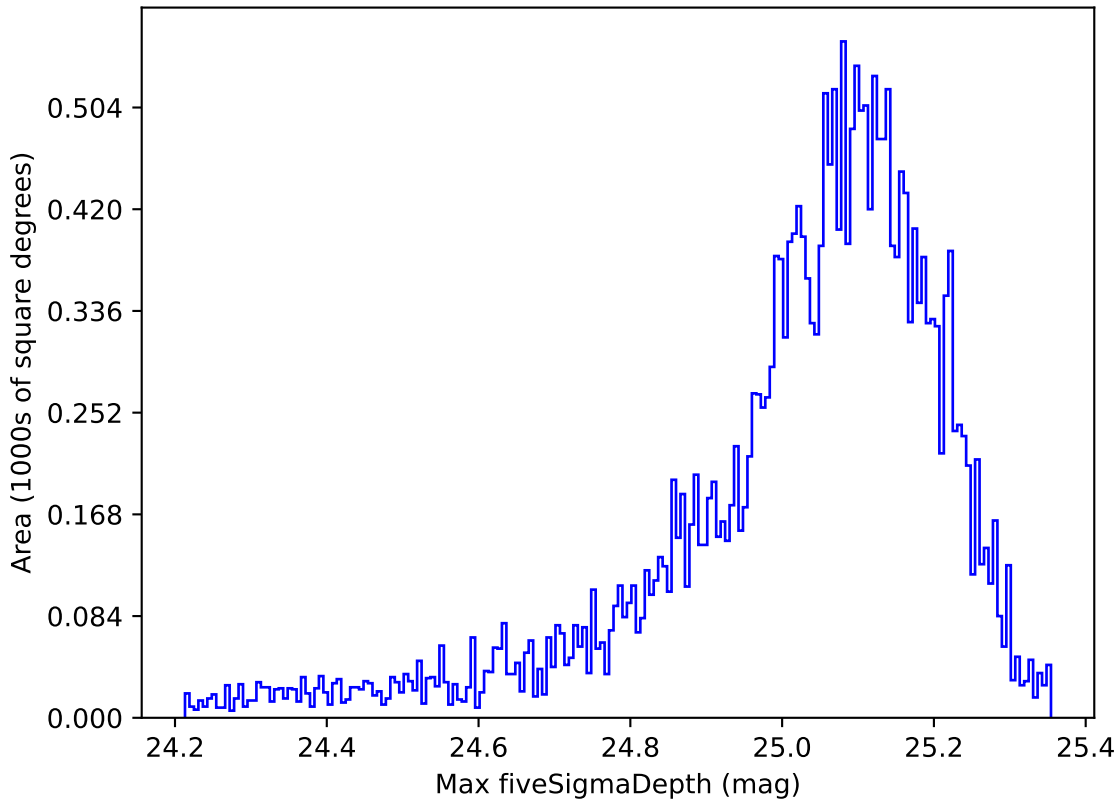
ddf_acor_sf15_lsf20_lsr50_v3.4_10yrs All sky g band: Max fiveSigmaDepth
