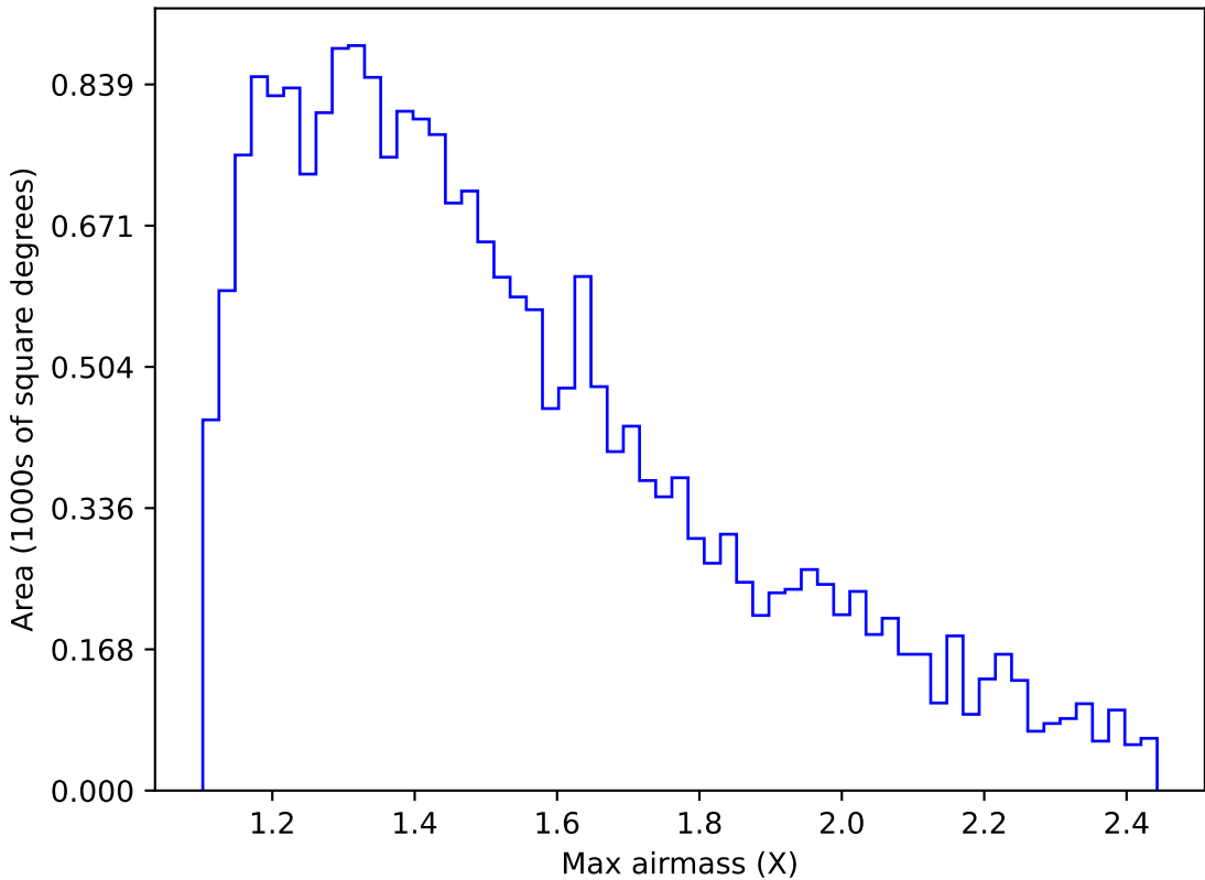
ddf_acor_sf15_lsf20_lsr50_v3.4_10yrs Yr 1 u band: Max airmass
