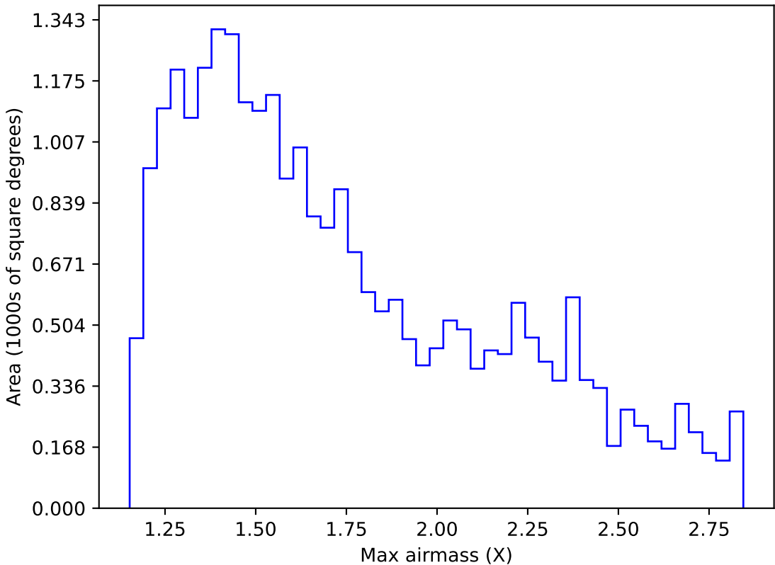
ddf_acor_sf15_lsf20_lsr50_v3.4_10yrs Yr 1 i band: Max airmass
