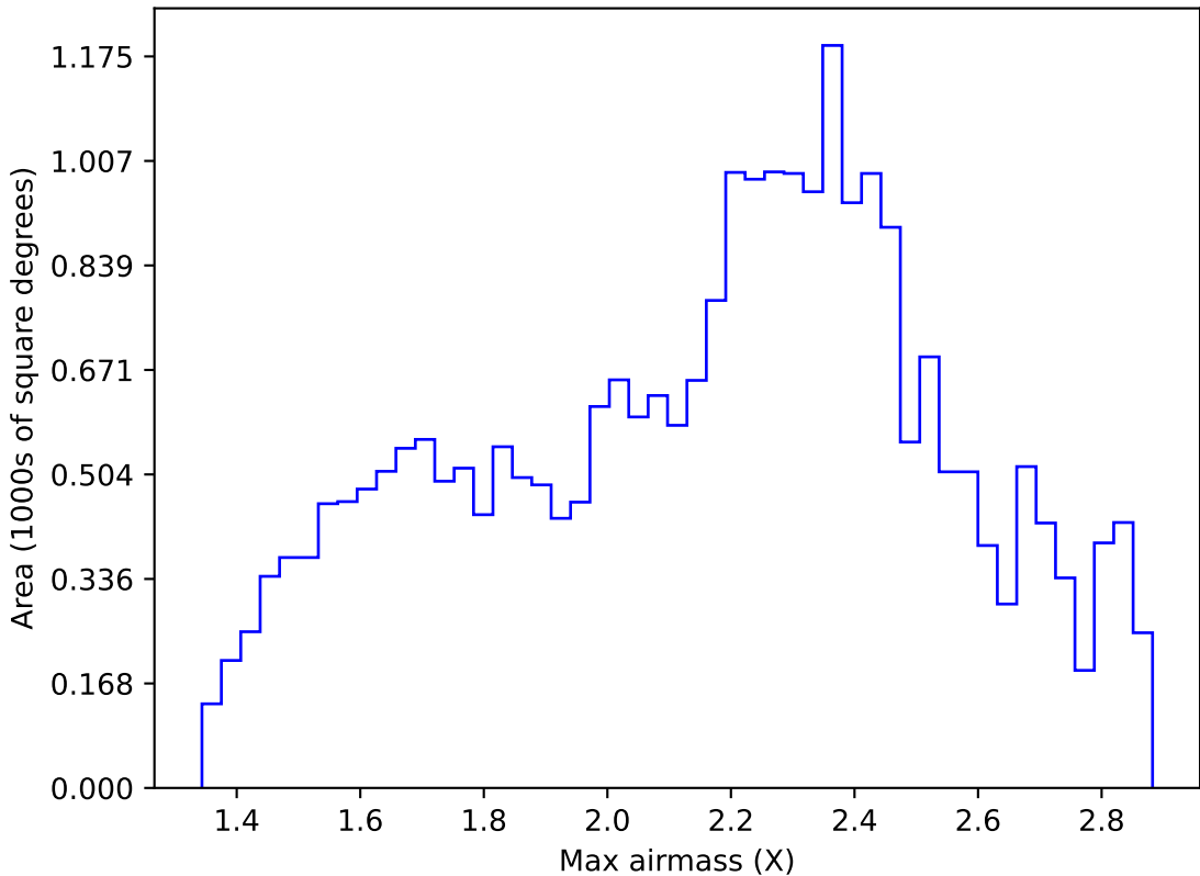
ddf_acor_sf15_lsf20_lsr50_v3.4_10yrs Yr 1 all bands: Max airmass
