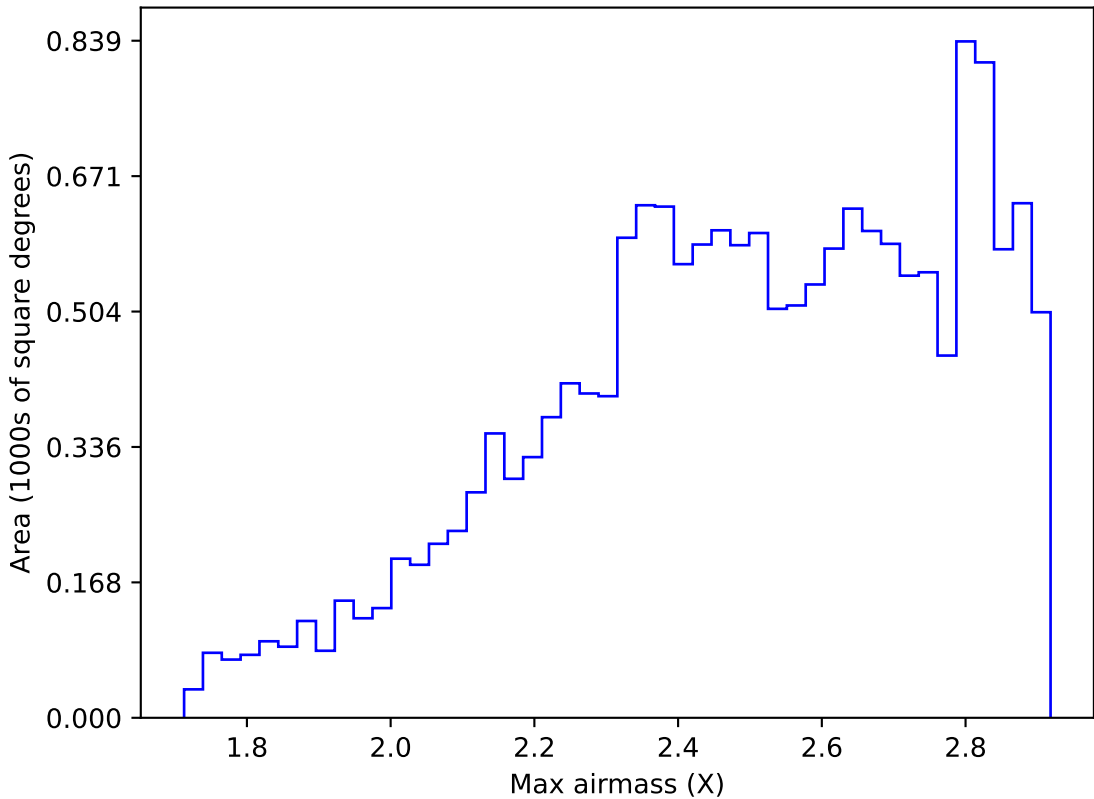
ddf_acor_sf15_lsf20_lsr50_v3.4_10yrs WFD i band: Max airmass
