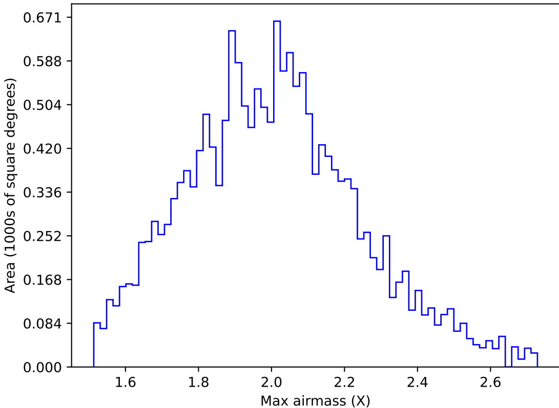
ddf_acor_sf15_lsf20_lsr50_v3.4_10yrs WFD g band: Max airmass
