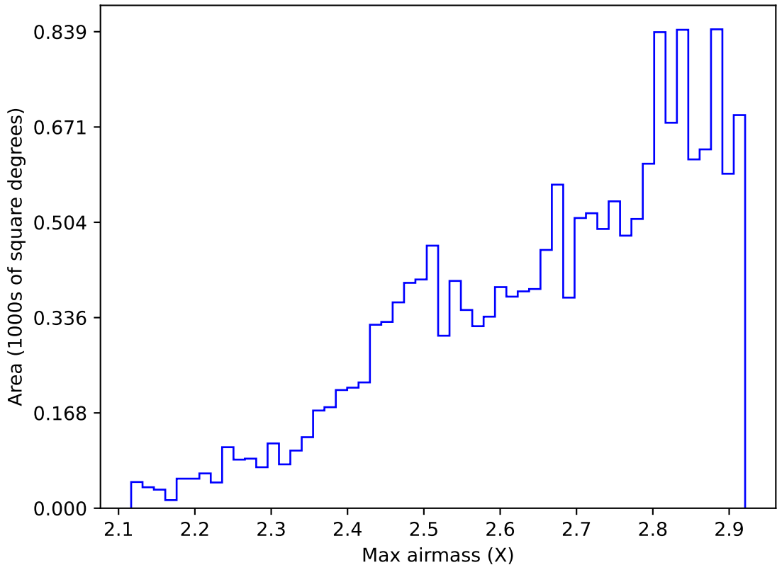
ddf_acor_sf15_lsf20_lsr50_v3.4_10yrs WFD all bands: Max airmass
