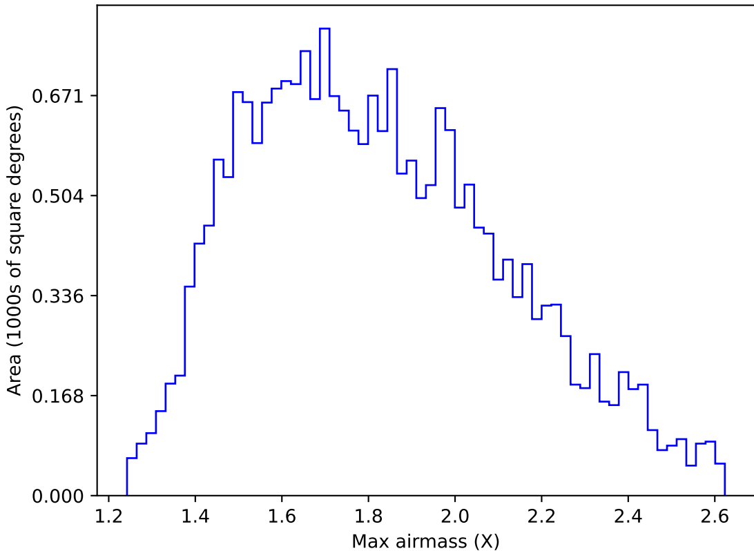
ddf_acor_sf15_lsf20_lsr50_v3.4_10yrs All sky u band: Max airmass
