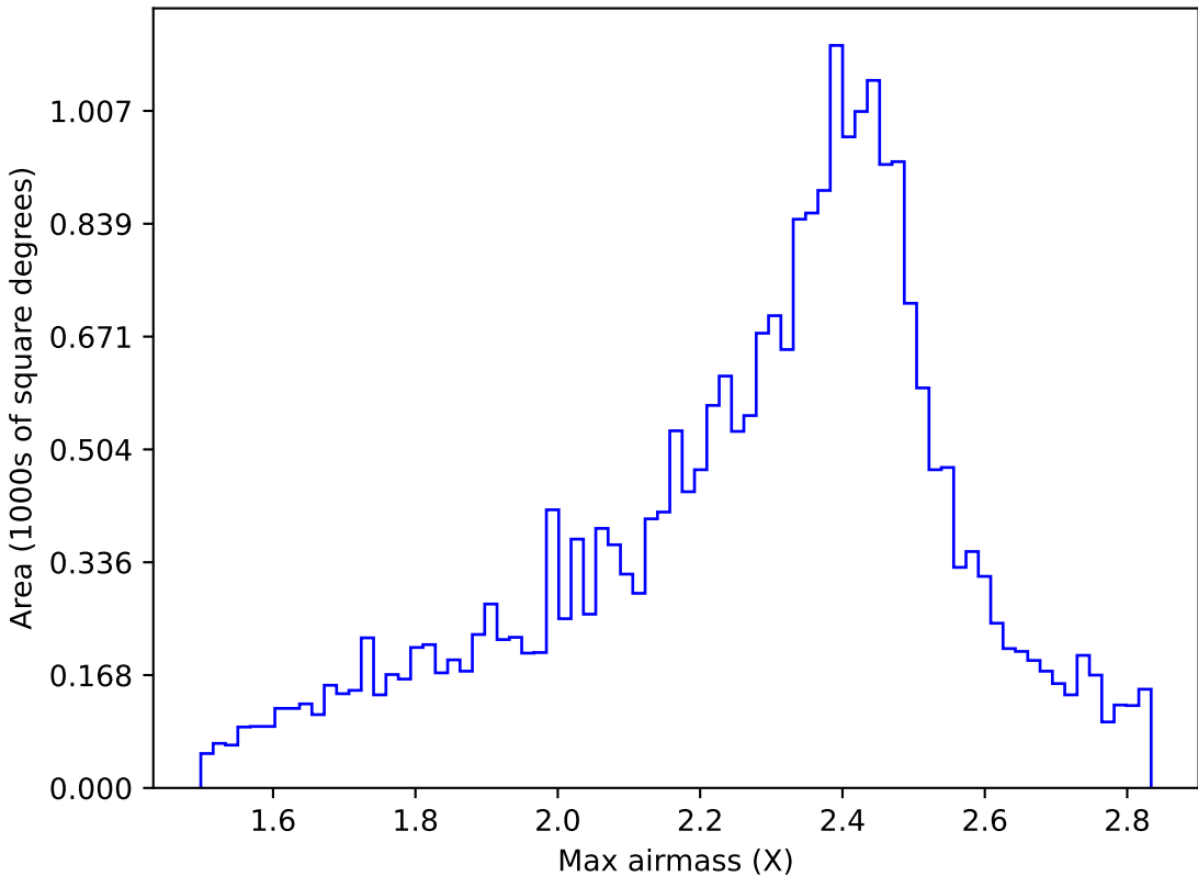
ddf_acor_sf15_lsf20_lsr50_v3.4_10yrs All sky r band: Max airmass
