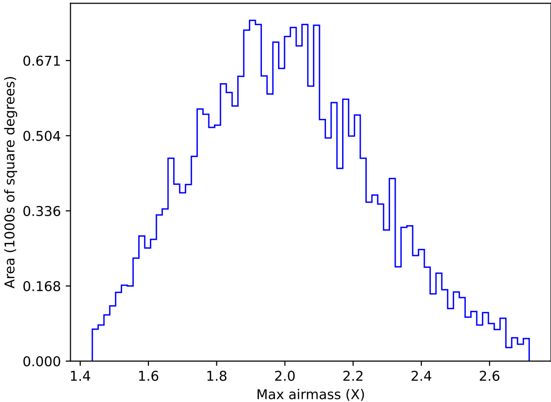
ddf_acor_sf15_lsf20_lsr50_v3.4_10yrs All sky g band: Max airmass
