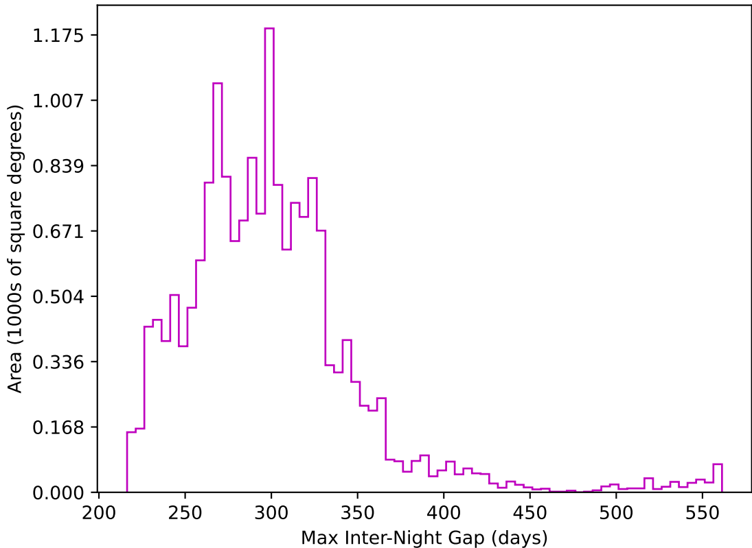
ddf_acor_sf15_lsf20_lsr50_v3.4_10yrs WFD z band: Max Inter-Night Gap
