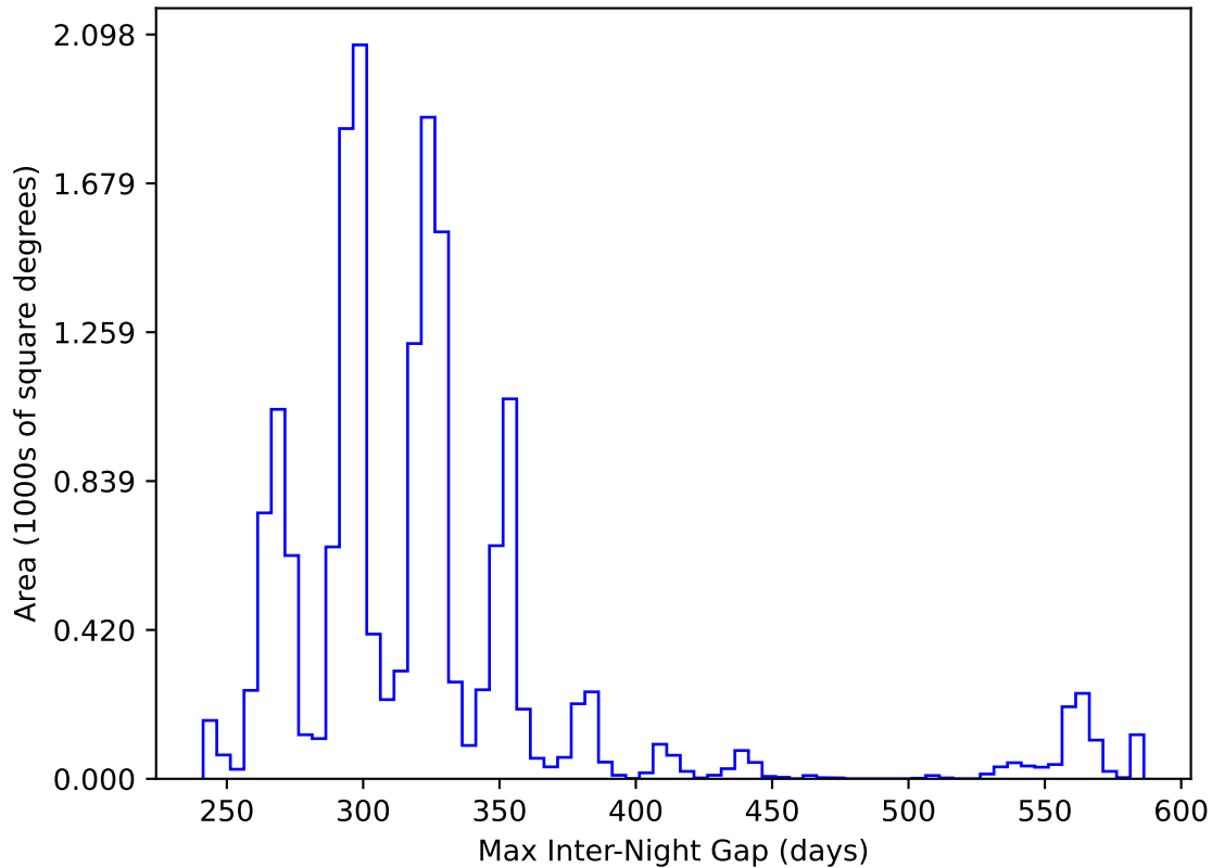
ddf_acor_sf15_lsf20_lsr50_v3.4_10yrs WFD y band: Max Inter-Night Gap
