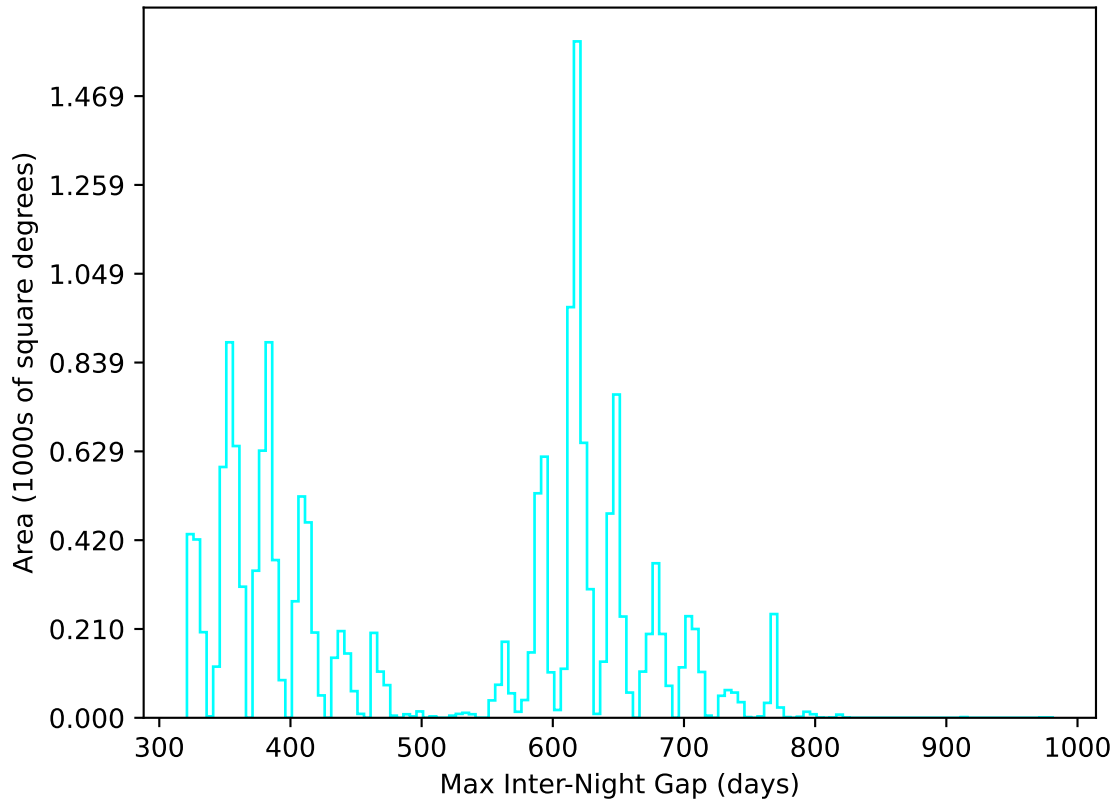
ddf_acor_sf15_lsf20_lsr50_v3.4_10yrs WFD u band: Max Inter-Night Gap
