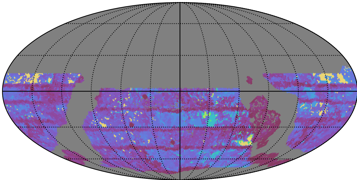
ddf_acor_sf15_lsf20_lsr50_v3.4_10yrs WFD r band: Max Inter-Night Gap
