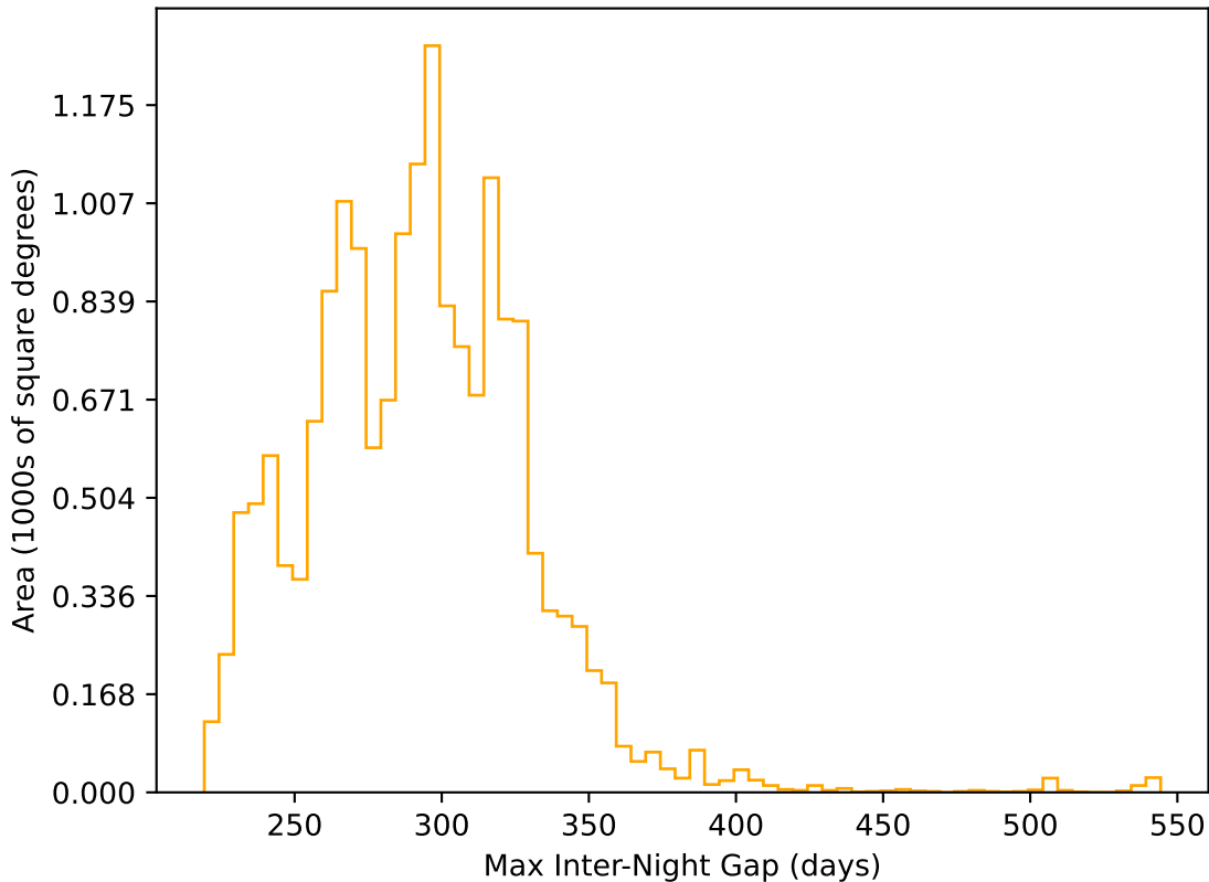
ddf_acor_sf15_lsf20_lsr50_v3.4_10yrs WFD r band: Max Inter-Night Gap
