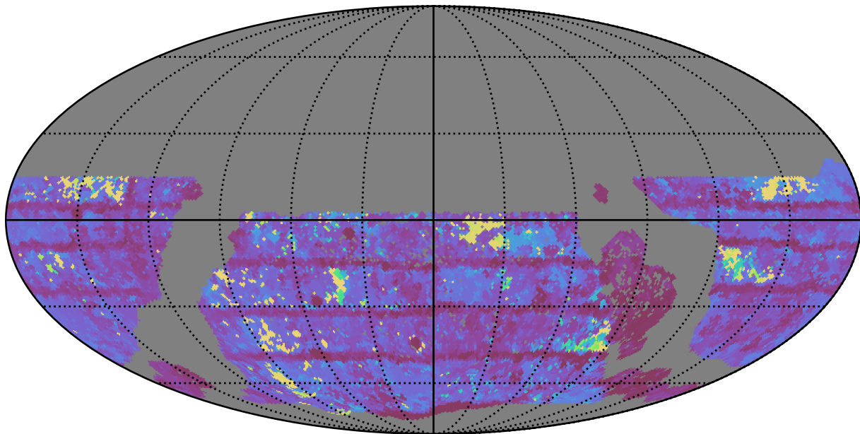
ddf_acor_sf15_lsf20_lsr50_v3.4_10yrs WFD i band: Max Inter-Night Gap
