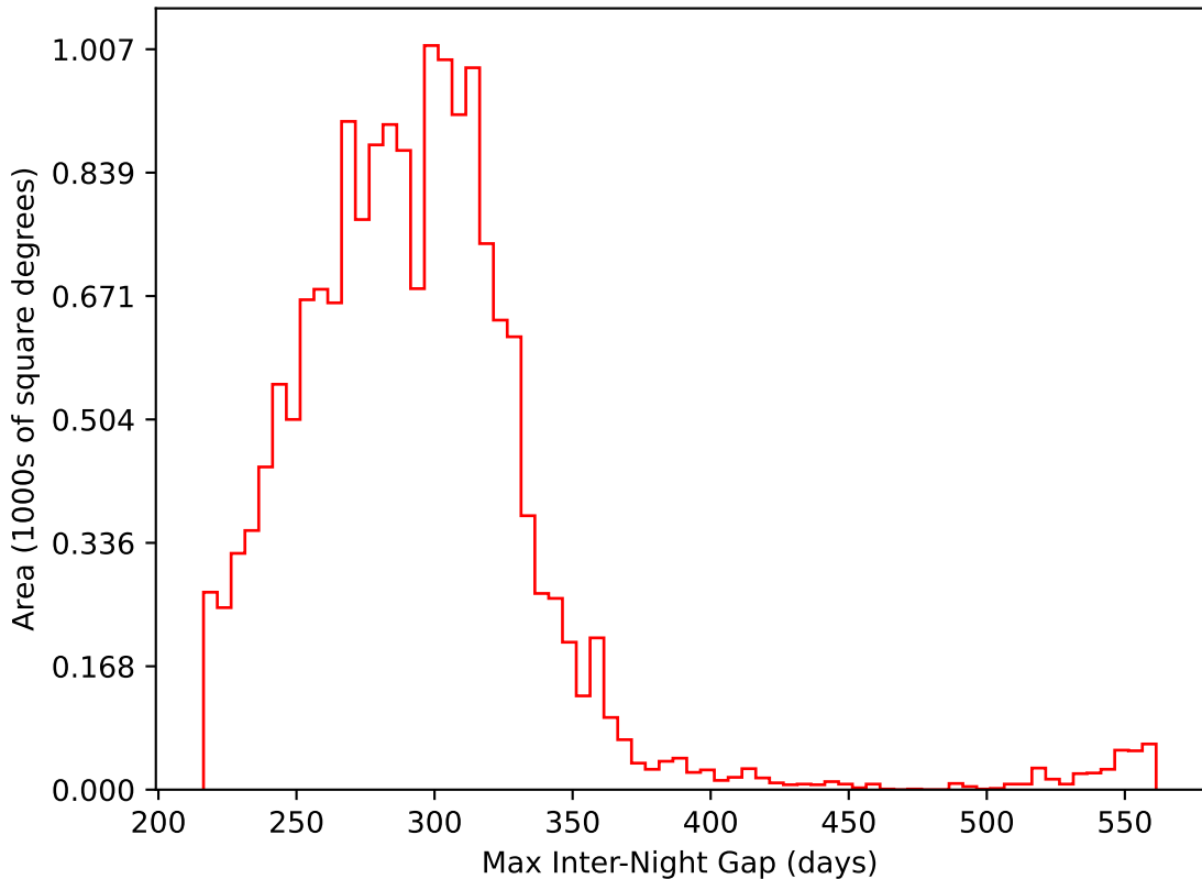
ddf_acor_sf15_lsf20_lsr50_v3.4_10yrs WFD i band: Max Inter-Night Gap
