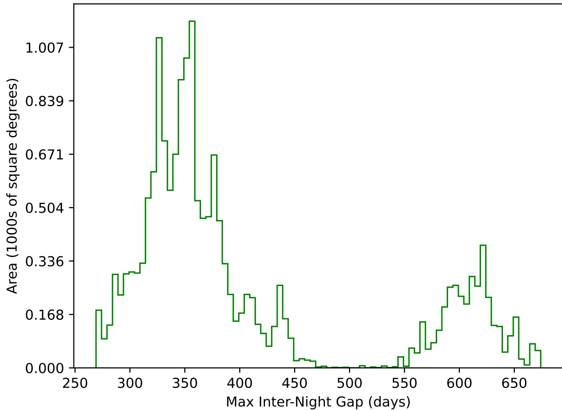
ddf_acor_sf15_lsf20_lsr50_v3.4_10yrs WFD g band: Max Inter-Night Gap
