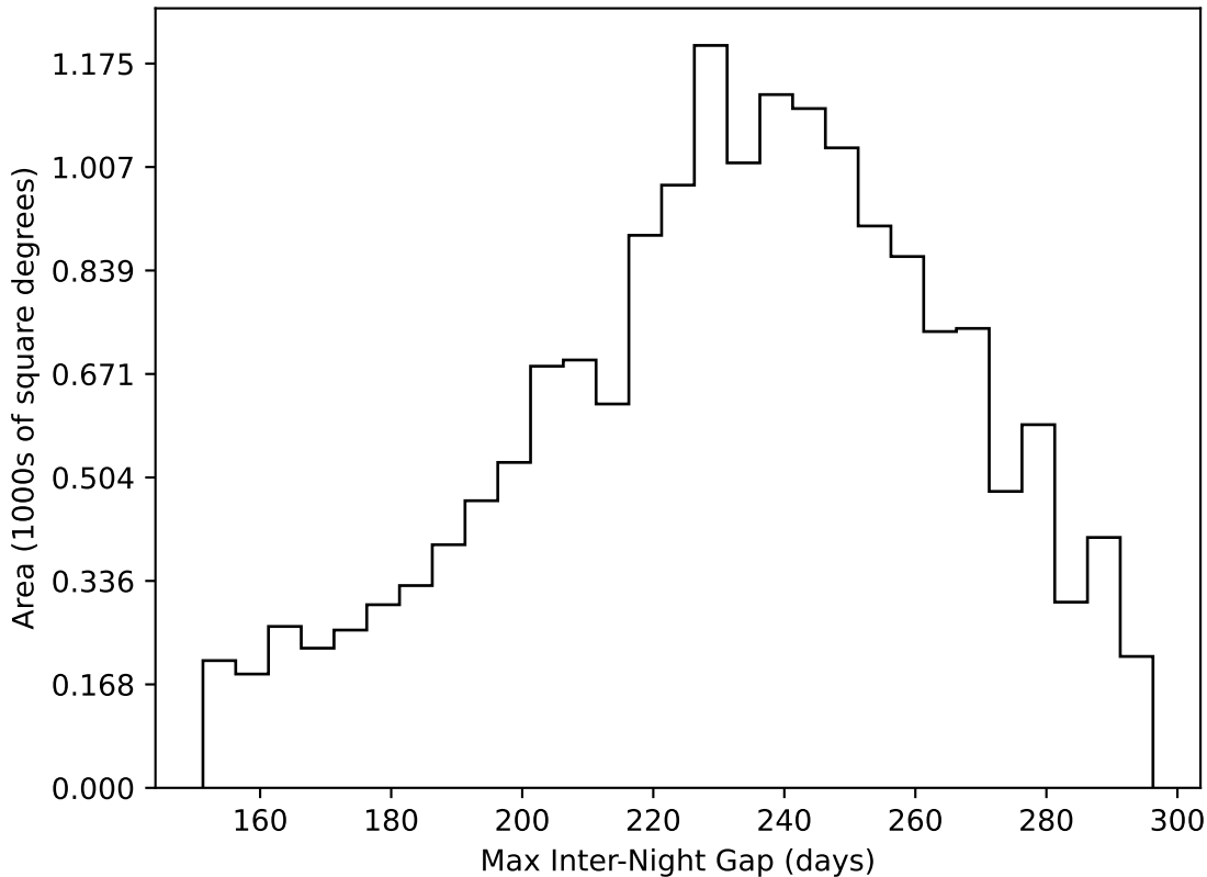
ddf_acor_sf15_lsf20_lsr50_v3.4_10yrs WFD all bands: Max Inter-Night Gap
