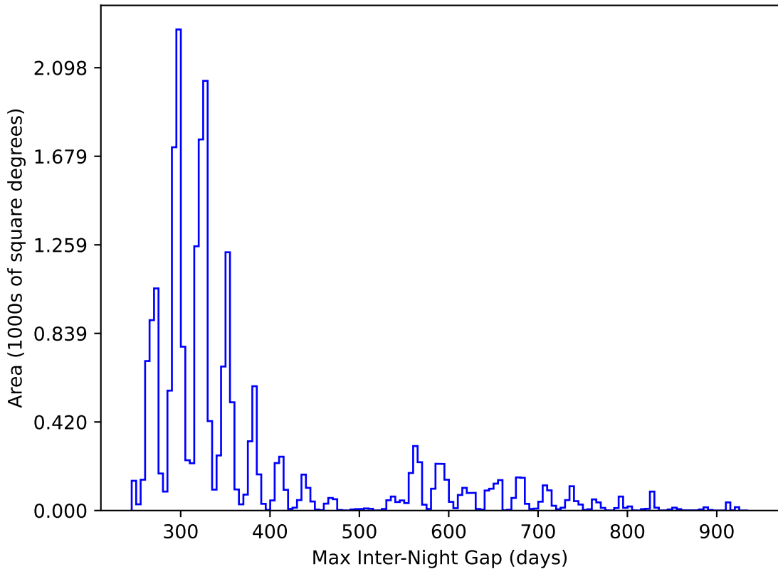
ddf_acor_sf15_lsf20_lsr50_v3.4_10yrs All sky y band: Max Inter-Night Gap
