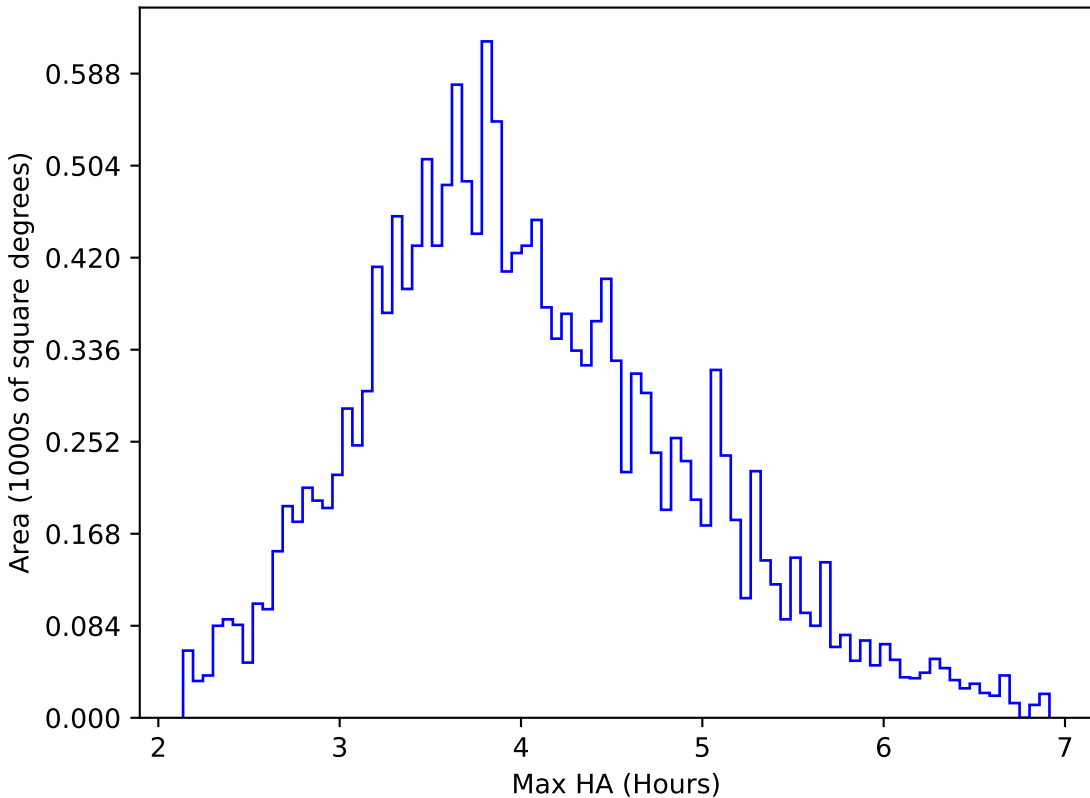
ddf_acor_sf15_lsf20_lsr50_v3.4_10yrs WFD g band: Max HA
