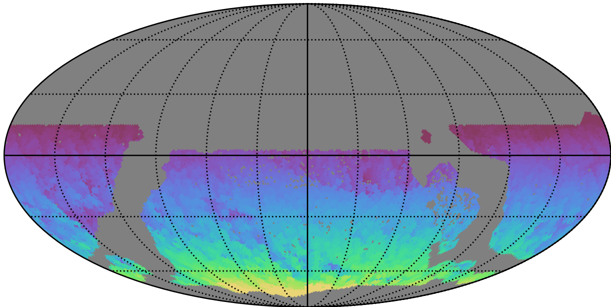
ddf_acor_sf15_lsf20_lsr50_v3.4_10yrs WFD all bands: Max HA
