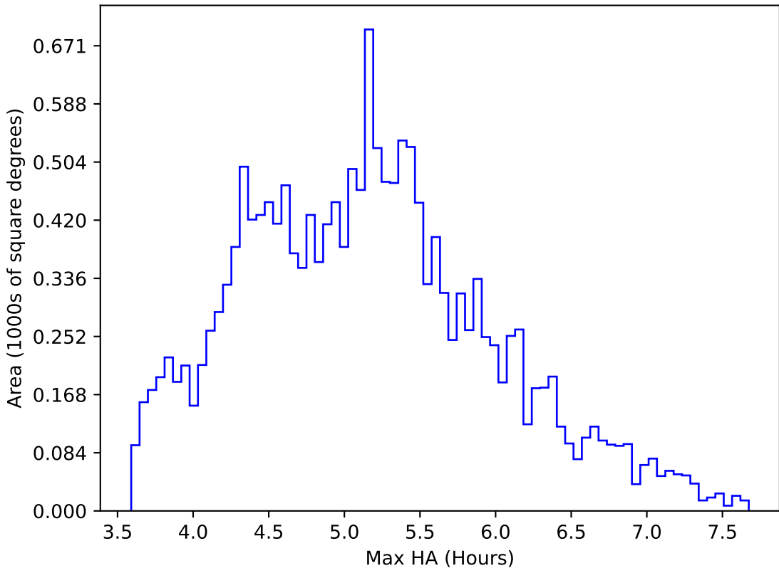
ddf_acor_sf15_lsf20_lsr50_v3.4_10yrs WFD all bands: Max HA
