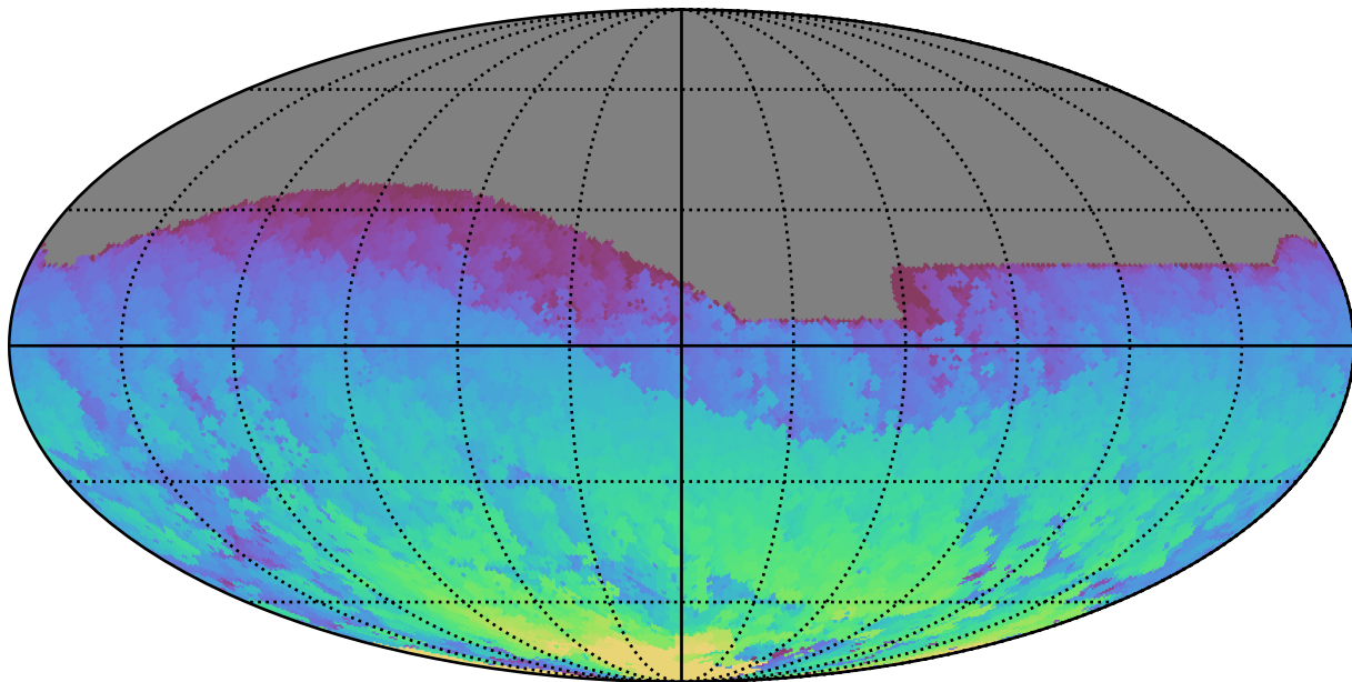
ddf_acor_sf15_lsf20_lsr50_v3.4_10yrs All sky z band: Max HA
